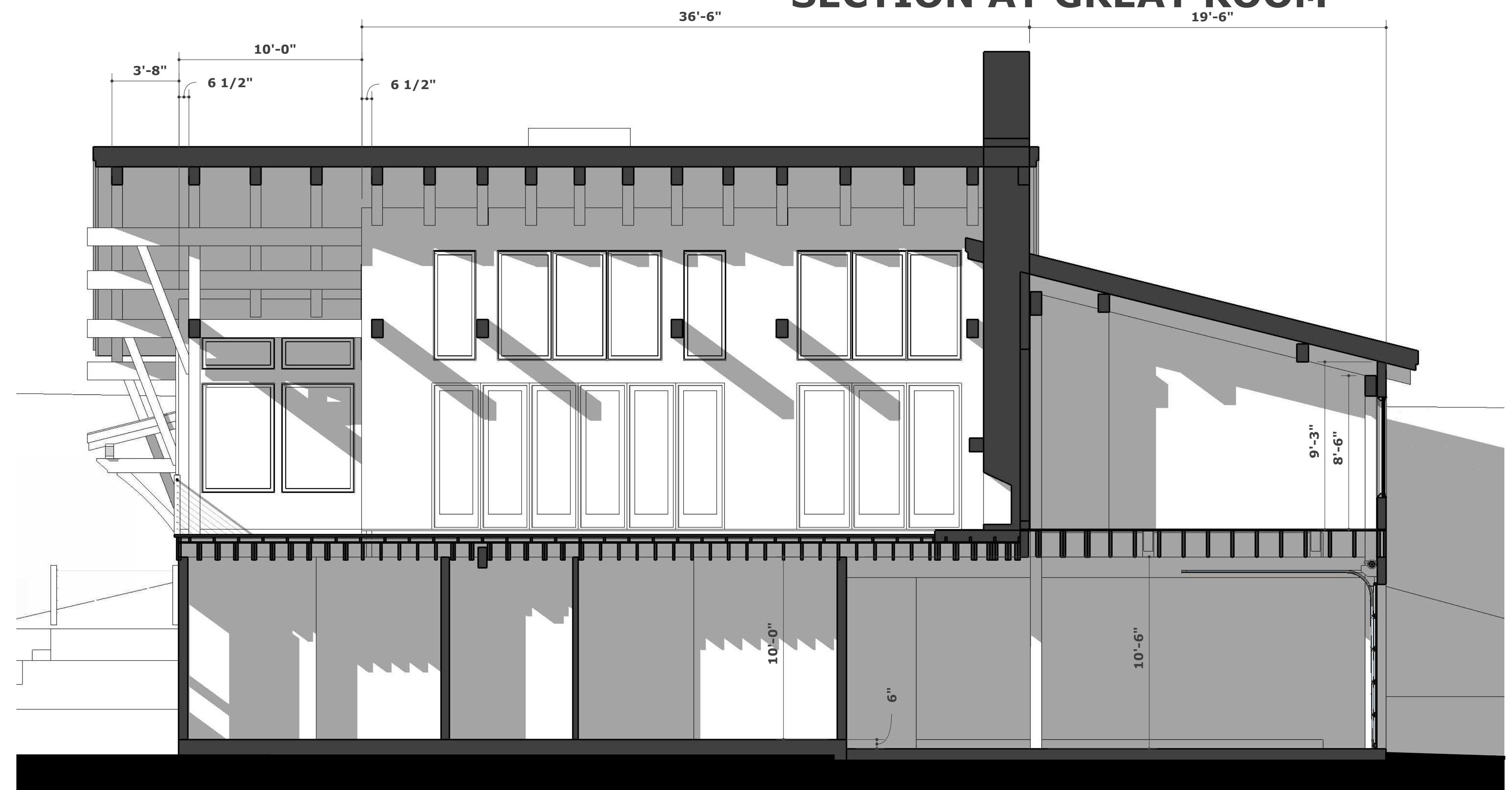
SECTION AT MASTER BEDROOM
