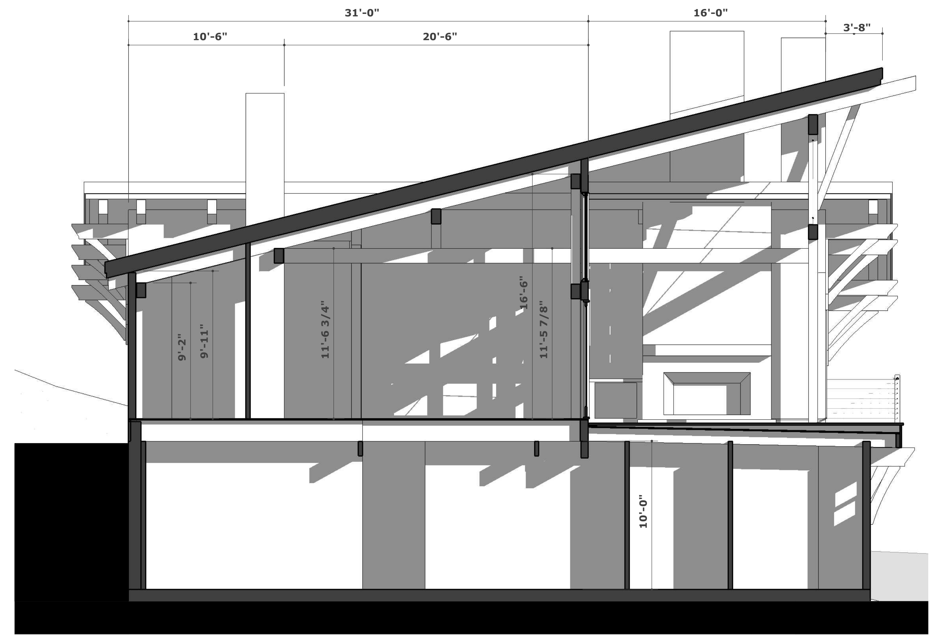
SECTION AT GREAT ROOM
