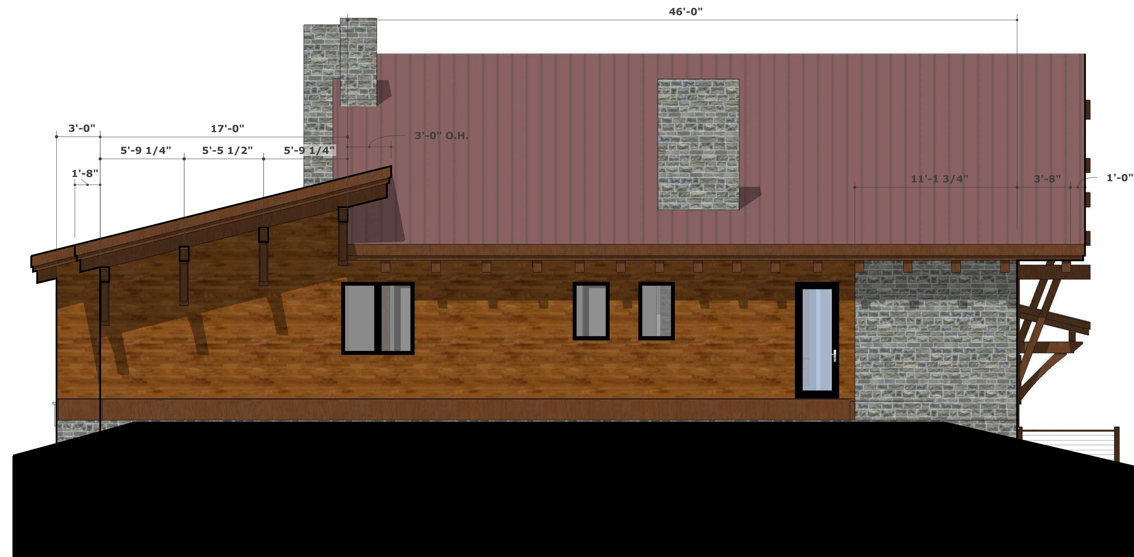
ENTRYSIDE (LEFT SIDE) ELEVATION
